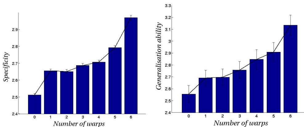
Figure x: Generalisability and Specificity of models with an increasing amount of deformation
